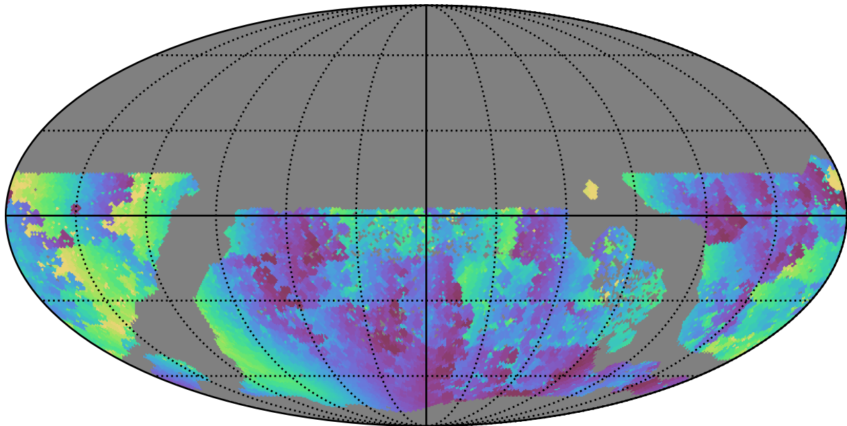
too_elab_r128_d2_gz_v3.4_10yrs WFD u band: Min solarElong
