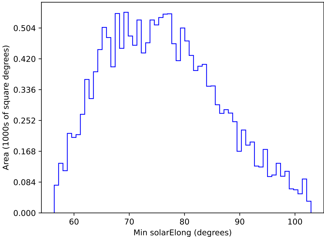
too_elab_r128_d2_gz_v3.4_10yrs WFD u band: Min solarElong
