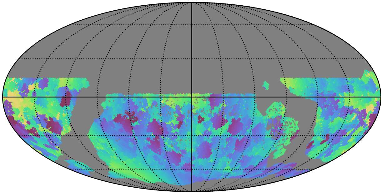
too_elab_r128_d2_gz_v3.4_10yrs WFD g band: Min solarElong
