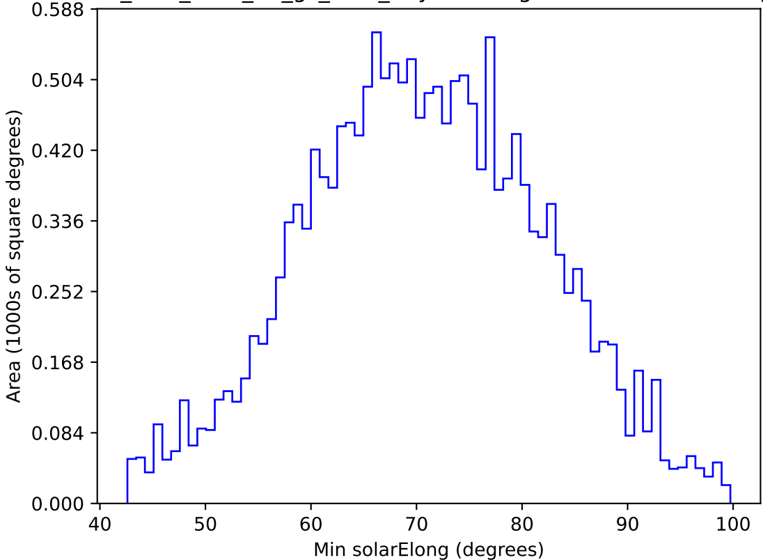
too_elab_r128_d2_gz_v3.4_10yrs WFD g band: Min solarElong
