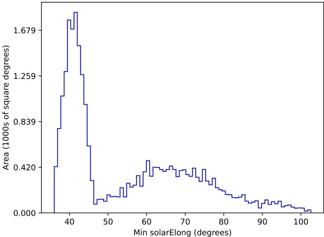
too_elab_r128_d2_gz_v3.4_10yrs All sky z band: Min solarElong
