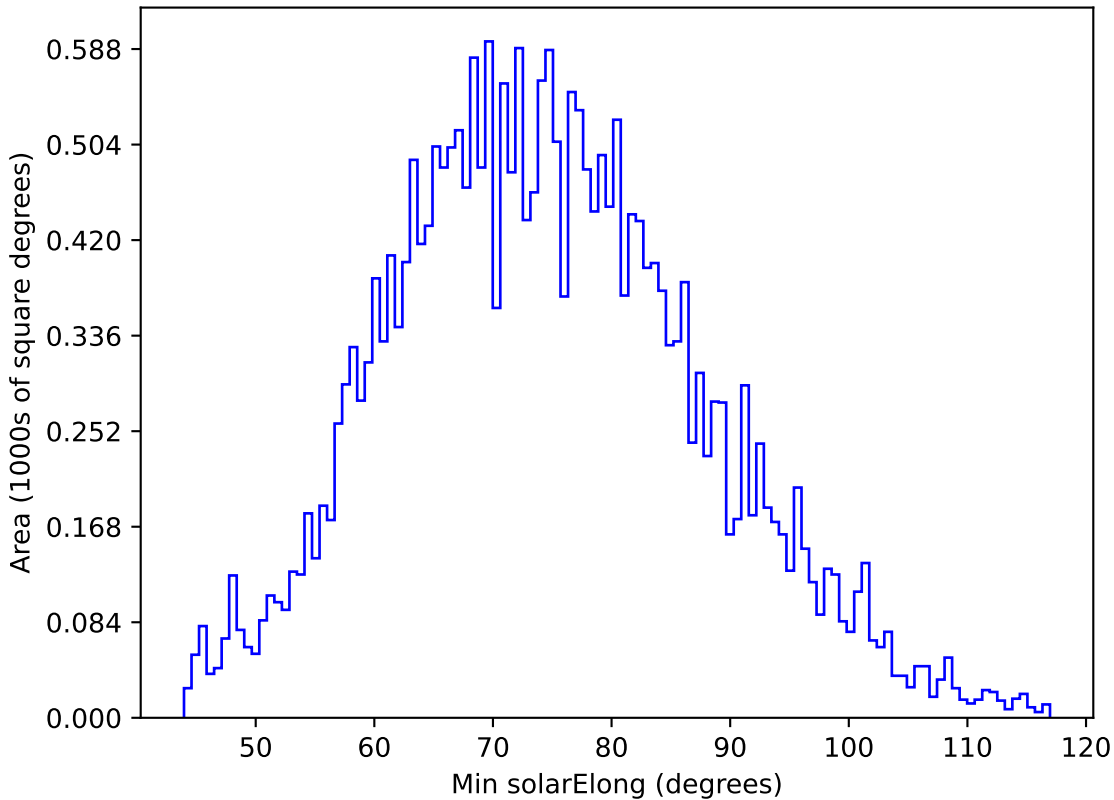
too_elab_r128_d2_gz_v3.4_10yrs All sky g band: Min solarElong
