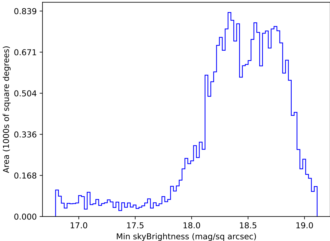
too_elab_r128_d2_gz_v3.4_10yrs Yr 1 z band: Min skyBrightness
