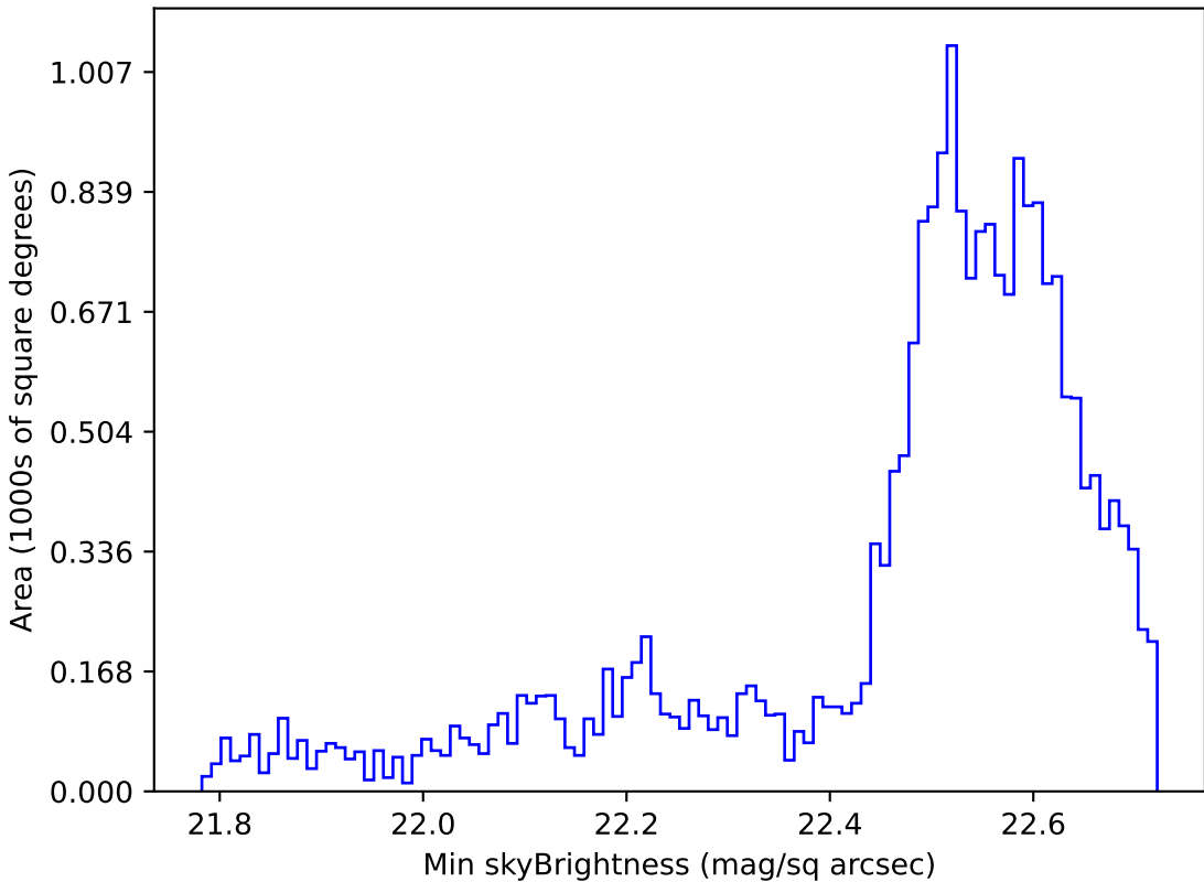
too_elab_r128_d2_gz_v3.4_10yrs Yr 1 u band: Min skyBrightness
