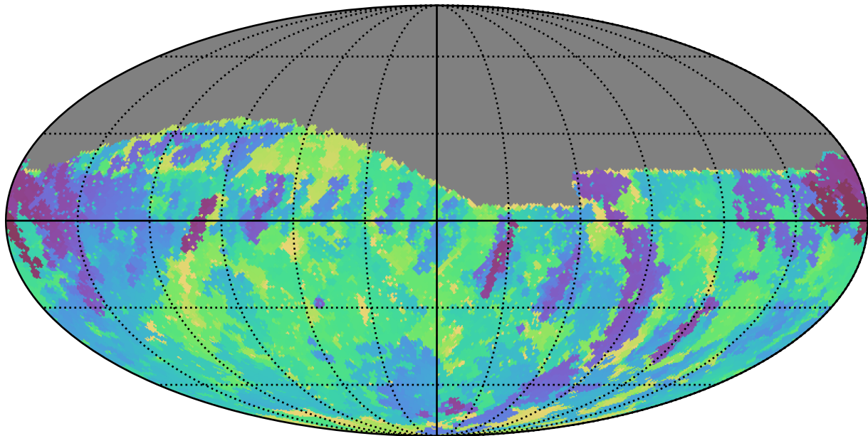
too_elab_r128_d2_gz_v3.4_10yrs Yr 1 r band: Min skyBrightness
