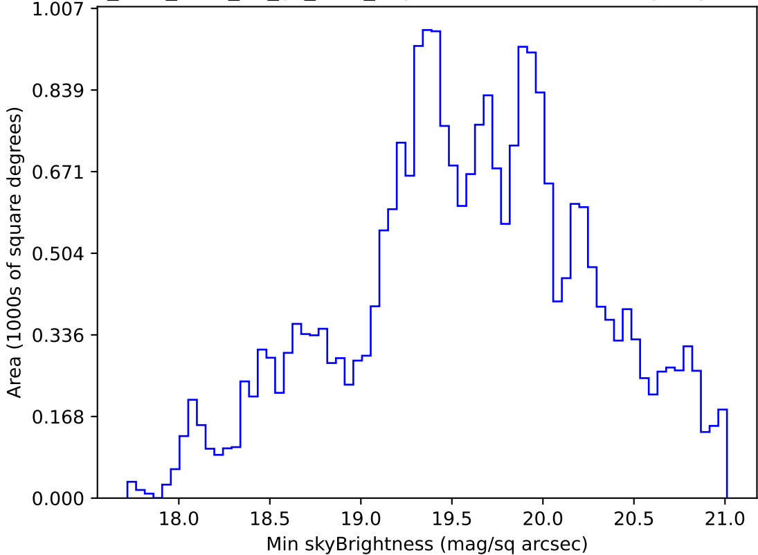
too_elab_r128_d2_gz_v3.4_10yrs Yr 1 r band: Min skyBrightness
