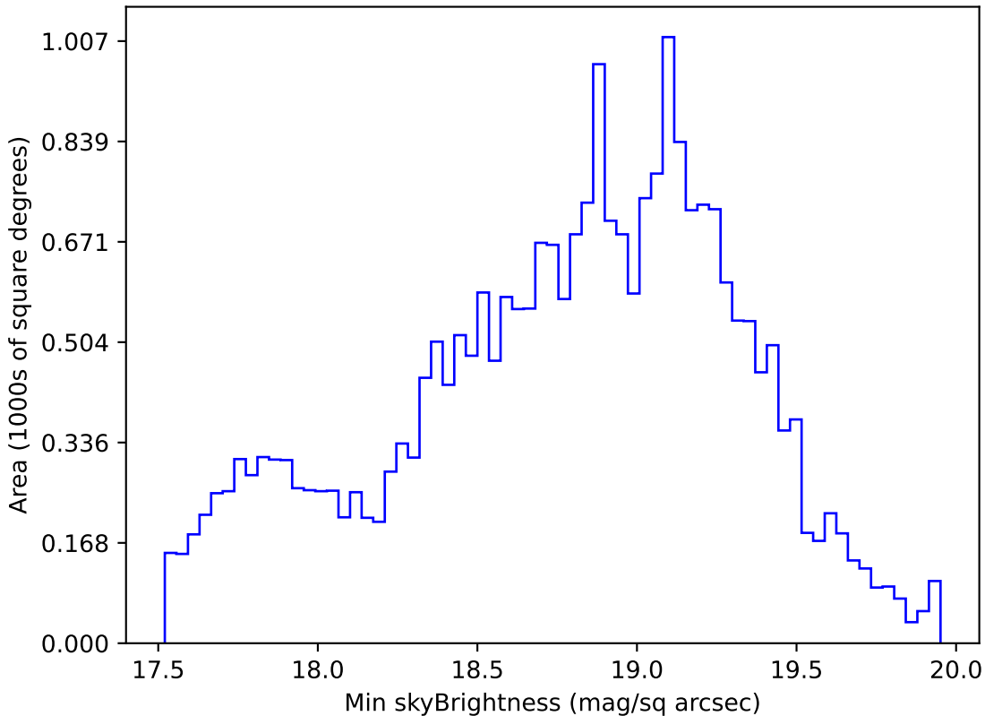
too_elab_r128_d2_gz_v3.4_10yrs Yr 1 i band: Min skyBrightness
