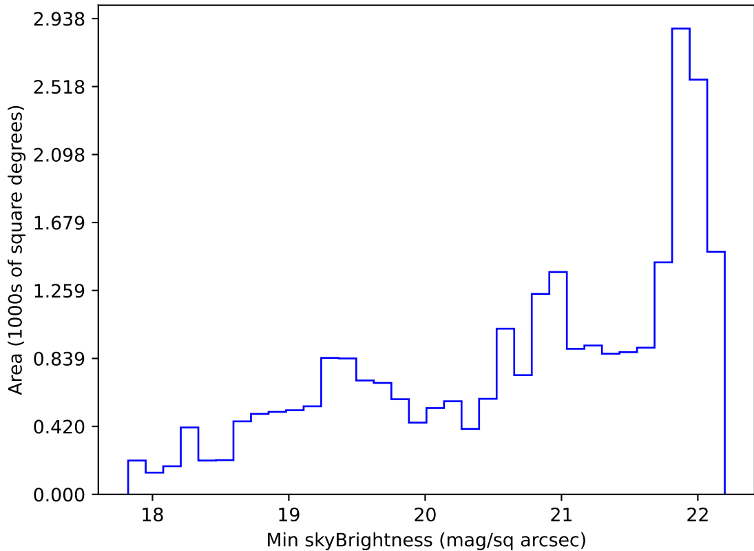
too_elab_r128_d2_gz_v3.4_10yrs Yr 1 g band: Min skyBrightness
