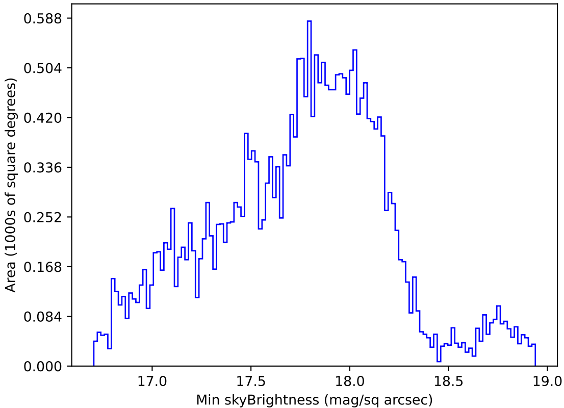
too_elab_r128_d2_gz_v3.4_10yrs Yr 1 all bands: Min skyBrightness
