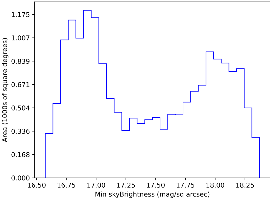
too_elab_r128_d2_gz_v3.4_10yrs WFD z band: Min skyBrightness
