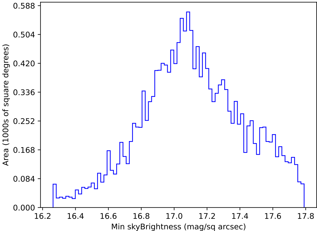
too_elab_r128_d2_gz_v3.4_10yrs WFD y band: Min skyBrightness
