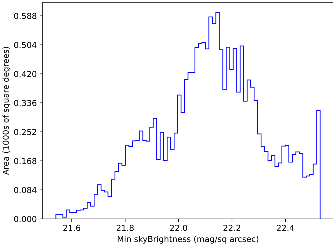
too_elab_r128_d2_gz_v3.4_10yrs WFD u band: Min skyBrightness
