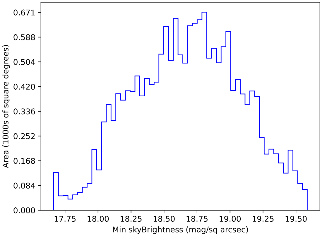
too_elab_r128_d2_gz_v3.4_10yrs WFD r band: Min skyBrightness
