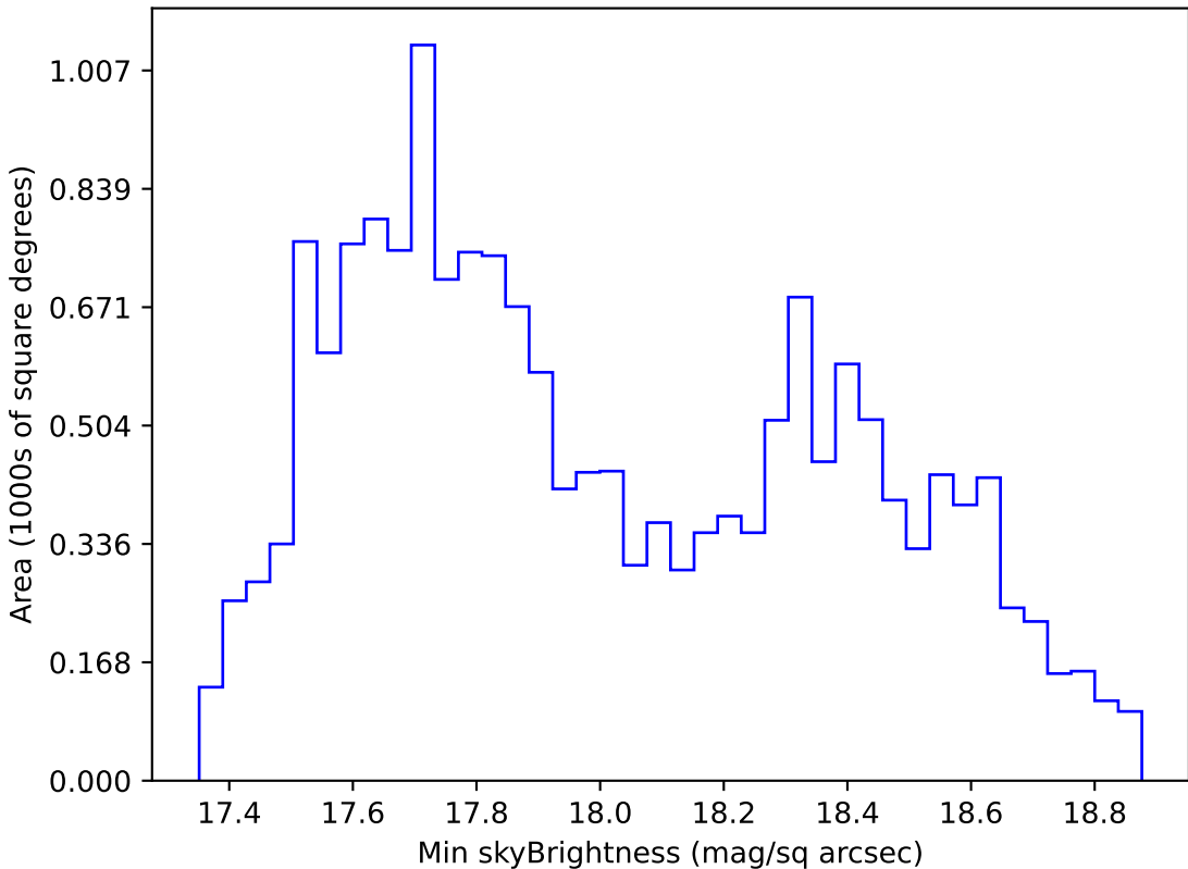
too_elab_r128_d2_gz_v3.4_10yrs WFD i band: Min skyBrightness
