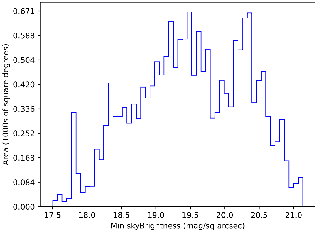
too_elab_r128_d2_gz_v3.4_10yrs WFD g band: Min skyBrightness
