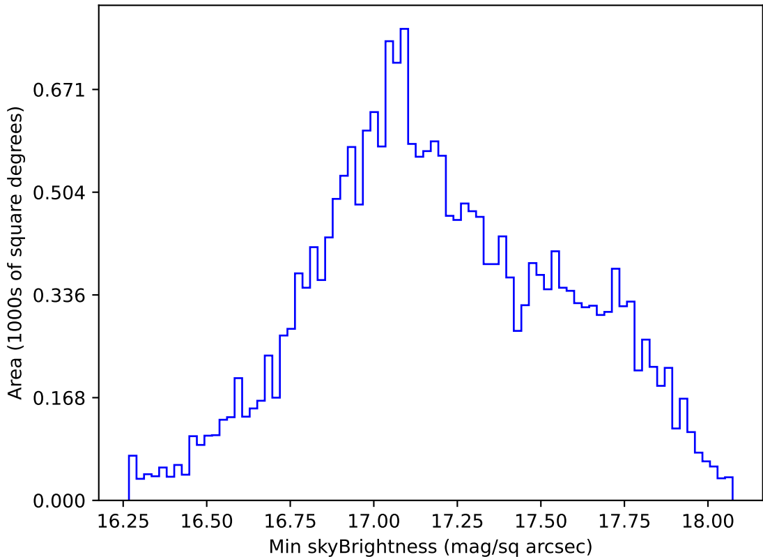
too_elab_r128_d2_gz_v3.4_10yrs All sky y band: Min skyBrightness
