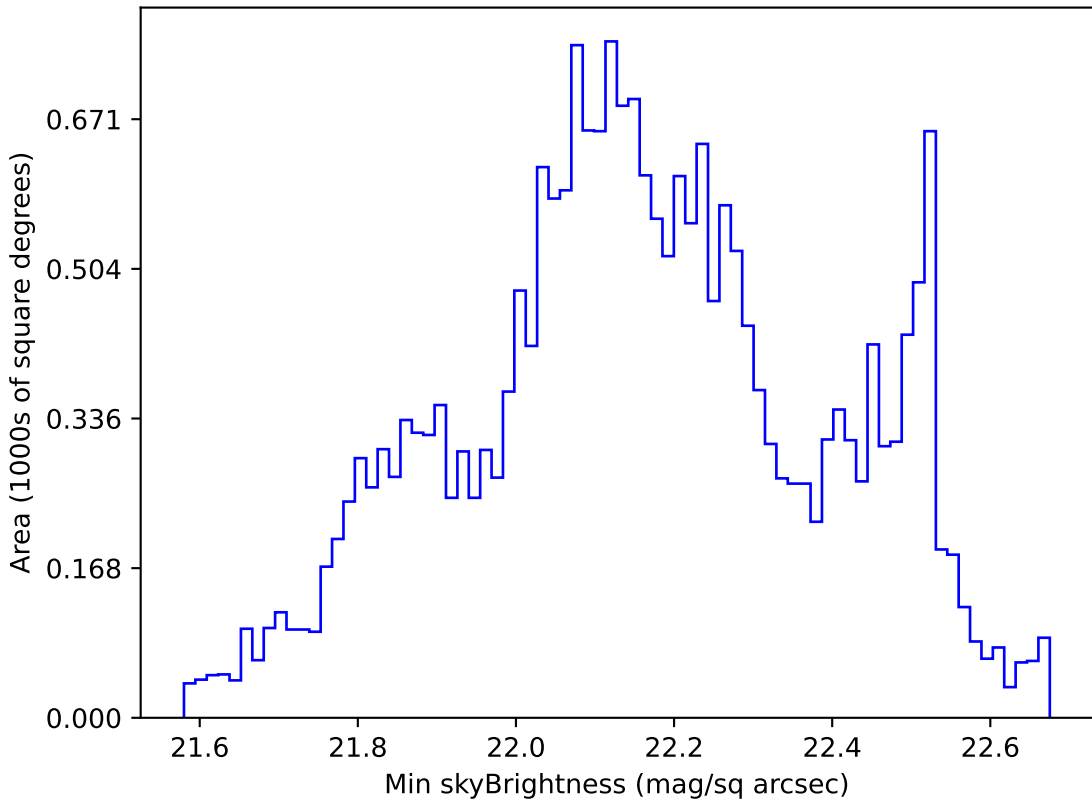
too_elab_r128_d2_gz_v3.4_10yrs All sky u band: Min skyBrightness
