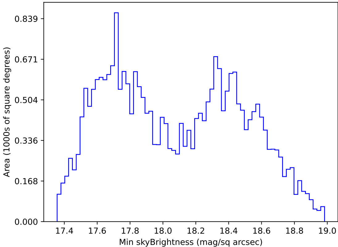
too_elab_r128_d2_gz_v3.4_10yrs All sky i band: Min skyBrightness
