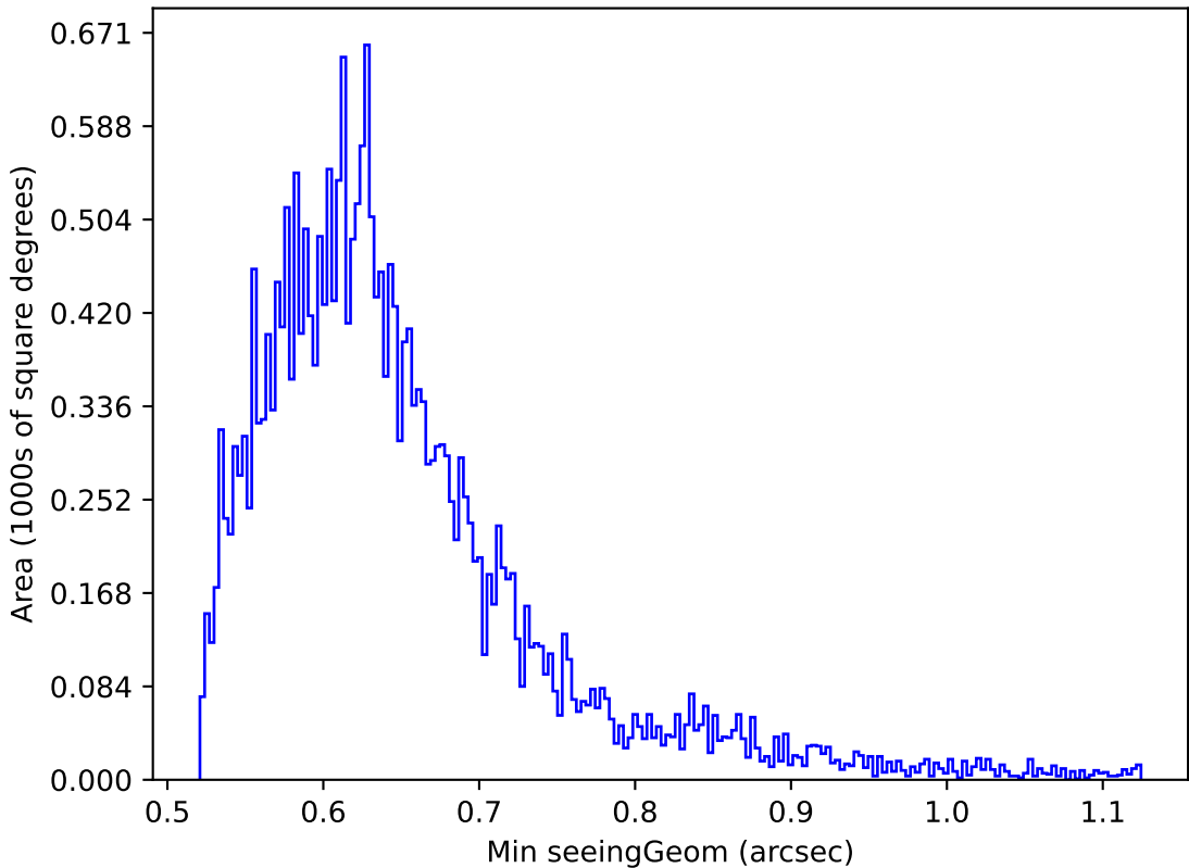
too_elab_r128_d2_gz_v3.4_10yrs Yr 1 z band: Min seeingGeom
