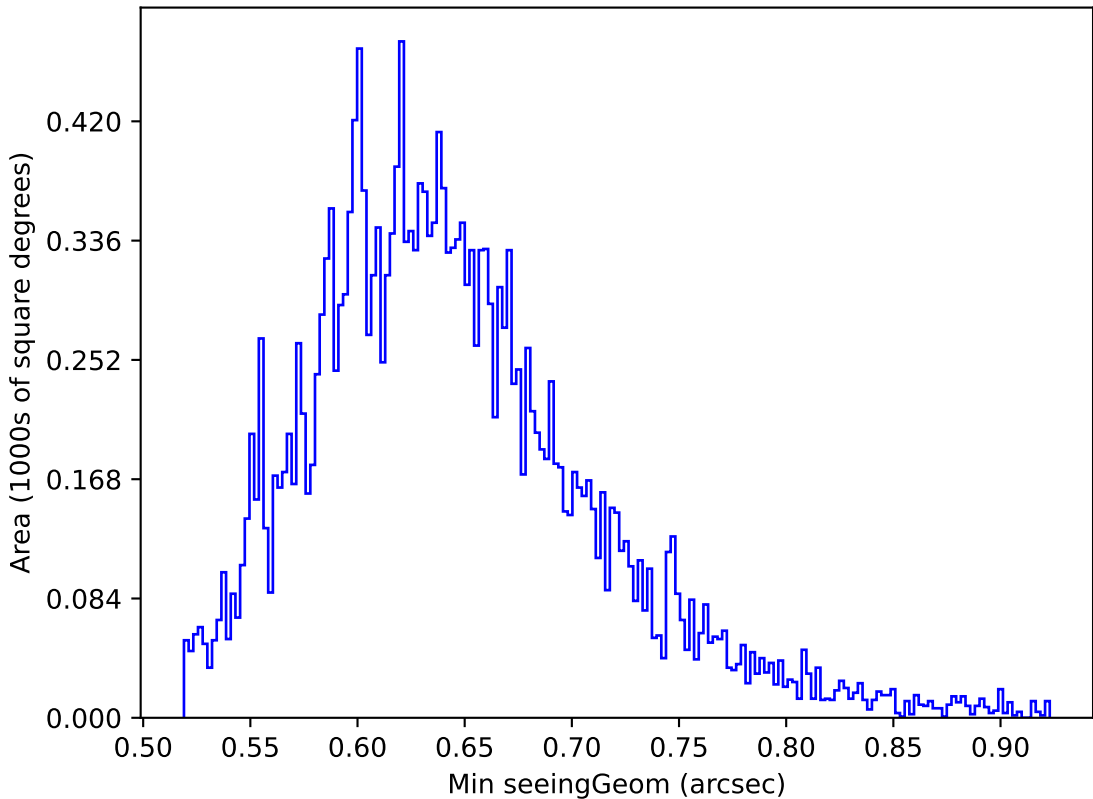
too_elab_r128_d2_gz_v3.4_10yrs Yr 1 y band: Min seeingGeom
