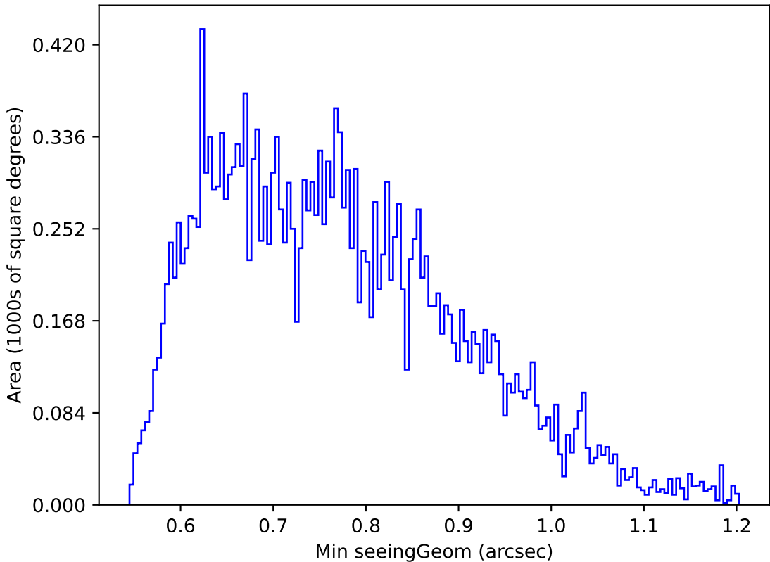
too_elab_r128_d2_gz_v3.4_10yrs Yr 1 u band: Min seeingGeom
