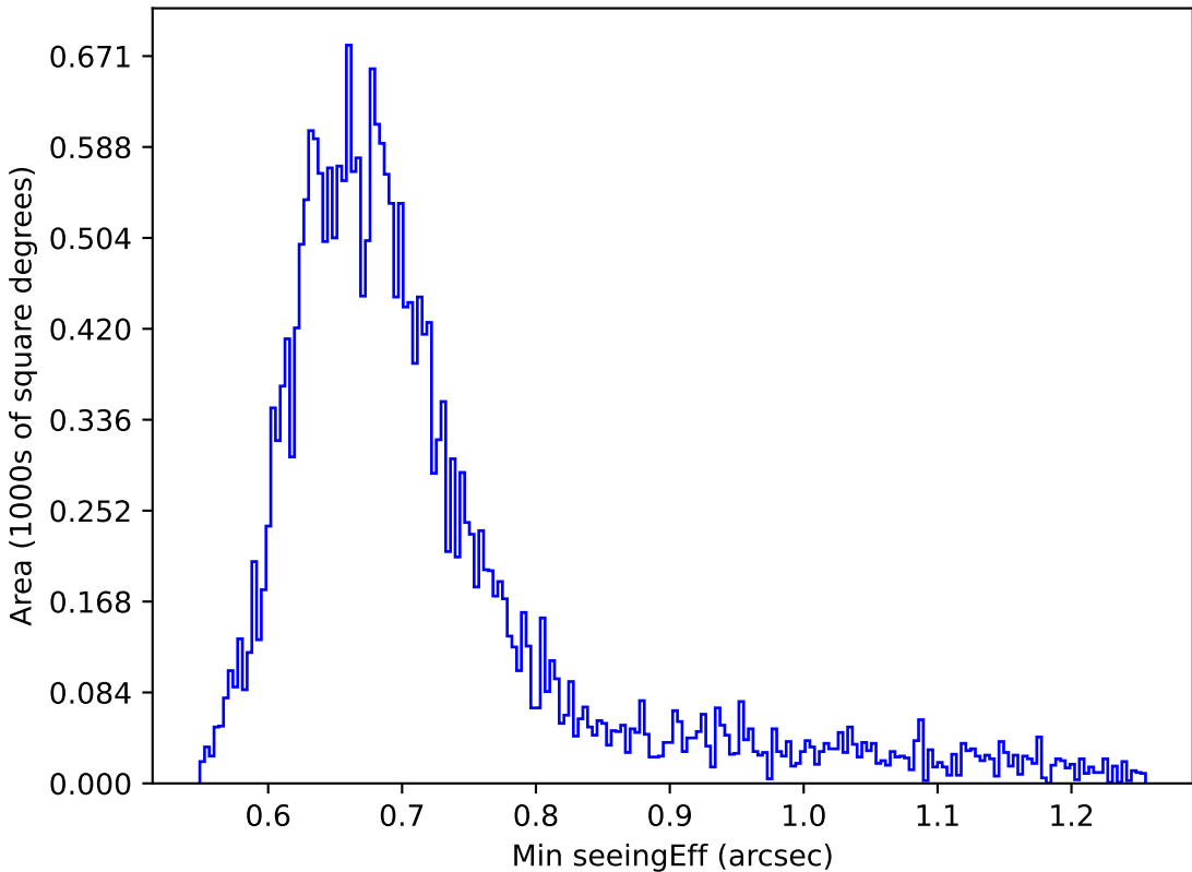
too_elab_r128_d2_gz_v3.4_10yrs Yr 1 r band: Min seeingEff
