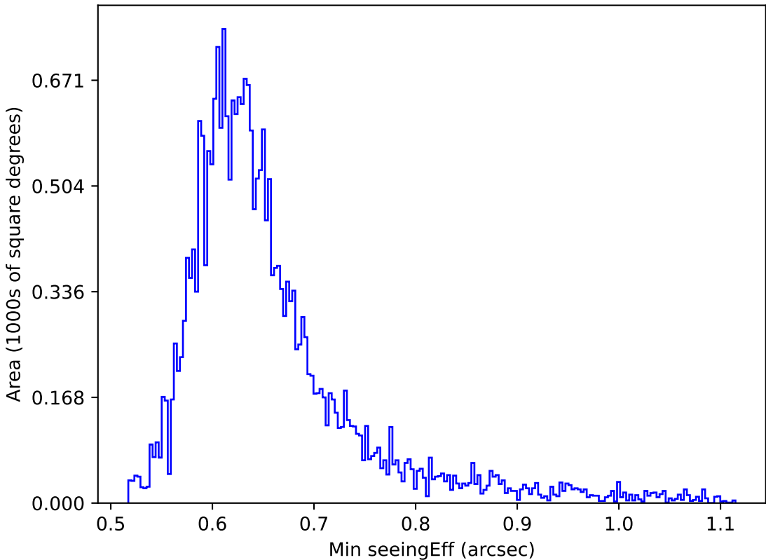
too_elab_r128_d2_gz_v3.4_10yrs Yr 1 all bands: Min seeingEff
