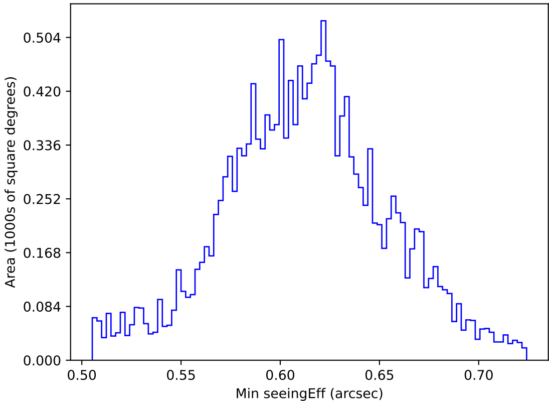
too_elab_r128_d2_gz_v3.4_10yrs WFD z band: Min seeingEff
