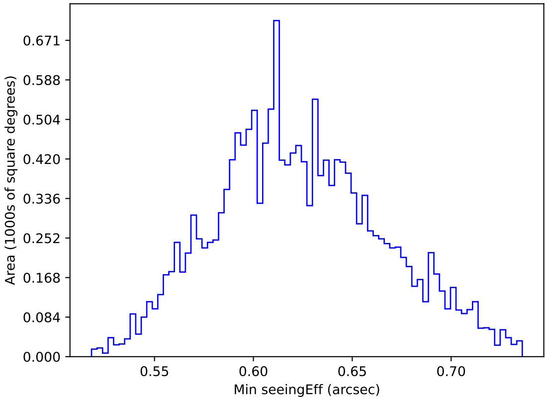
too_elab_r128_d2_gz_v3.4_10yrs WFD y band: Min seeingEff
