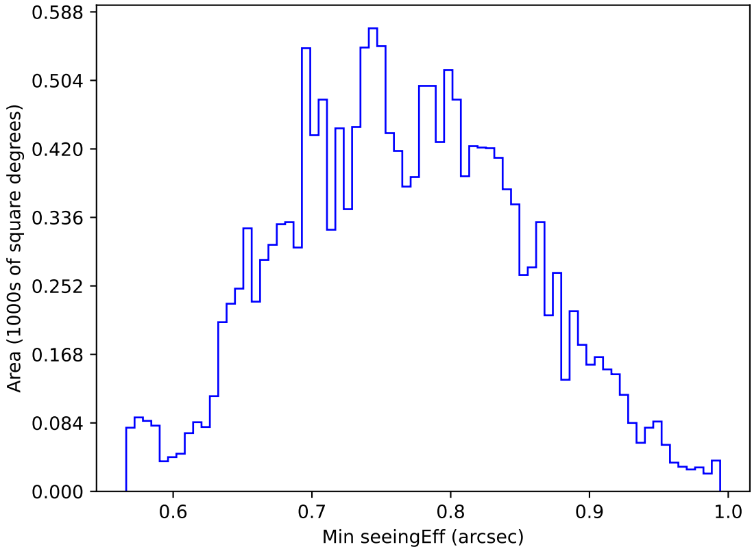
too_elab_r128_d2_gz_v3.4_10yrs WFD u band: Min seeingEff
