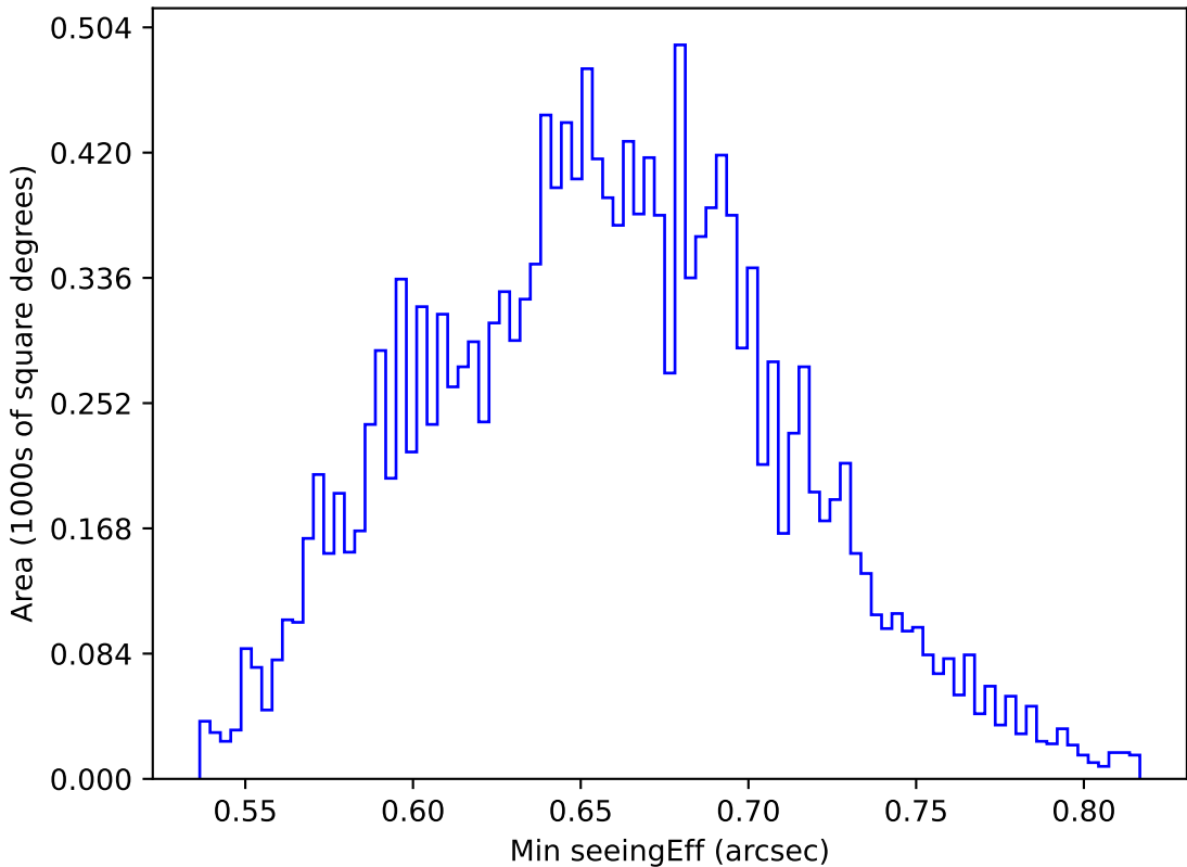
too_elab_r128_d2_gz_v3.4_10yrs WFD g band: Min seeingEff
