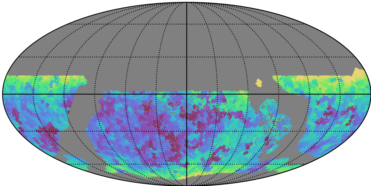
too_elab_r128_d2_gz_v3.4_10yrs WFD all bands: Min seeingEff
