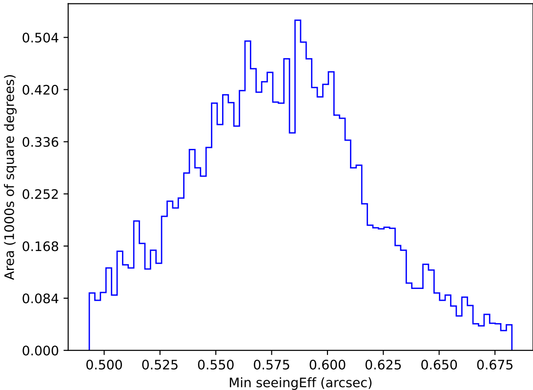
too_elab_r128_d2_gz_v3.4_10yrs WFD all bands: Min seeingEff
