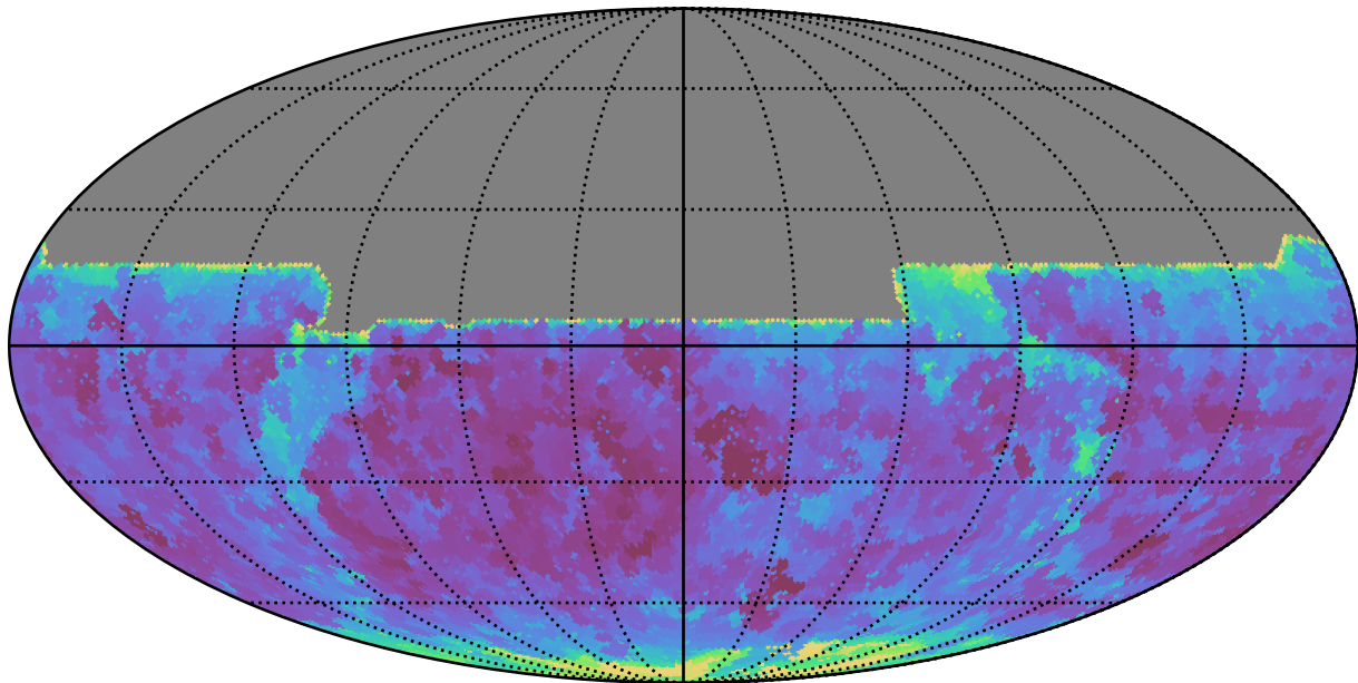
too_elab_r128_d2_gz_v3.4_10yrs All sky y band: Min seeingEff
