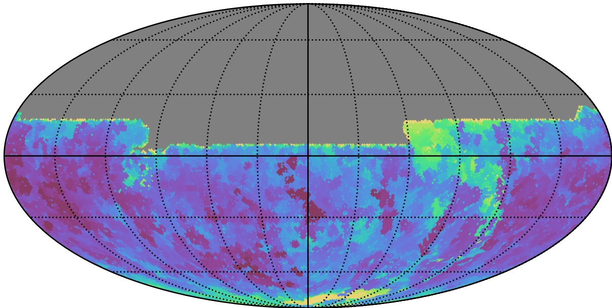
too_elab_r128_d2_gz_v3.4_10yrs All sky u band: Min seeingEff
