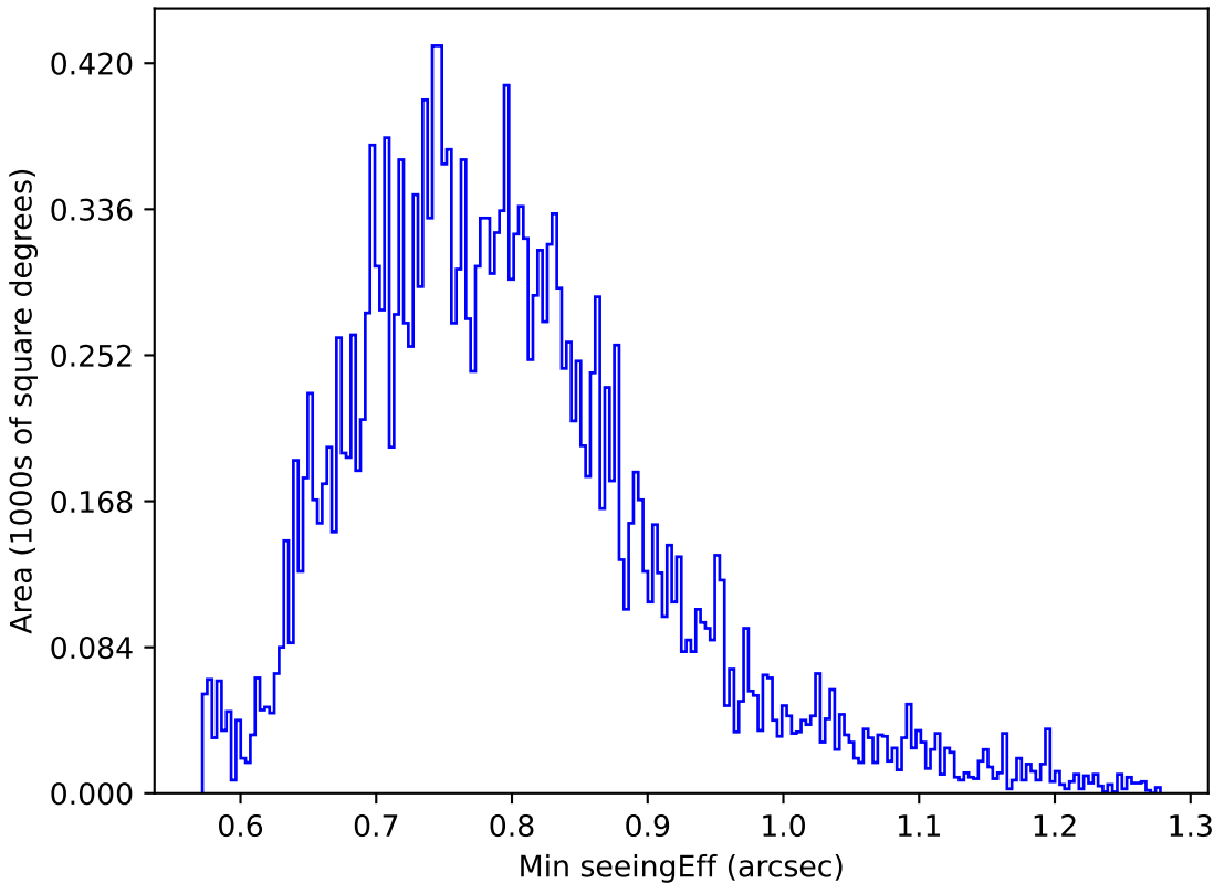
too_elab_r128_d2_gz_v3.4_10yrs All sky u band: Min seeingEff
