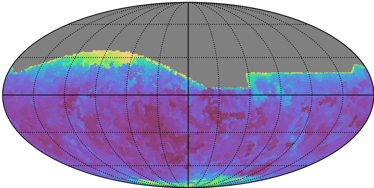
too_elab_r128_d2_gz_v3.4_10yrs All sky r band: Min seeingEff
