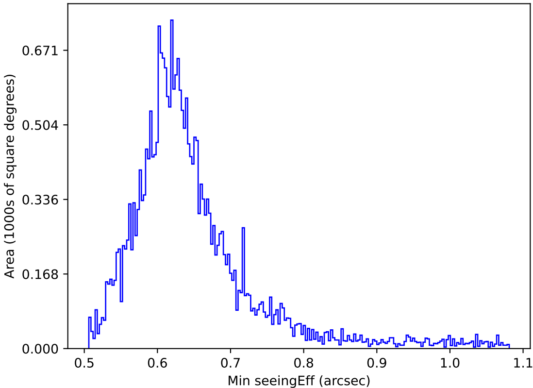
too_elab_r128_d2_gz_v3.4_10yrs All sky r band: Min seeingEff
