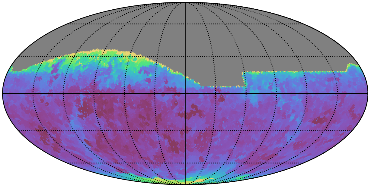
too_elab_r128_d2_gz_v3.4_10yrs All sky i band: Min seeingEff
