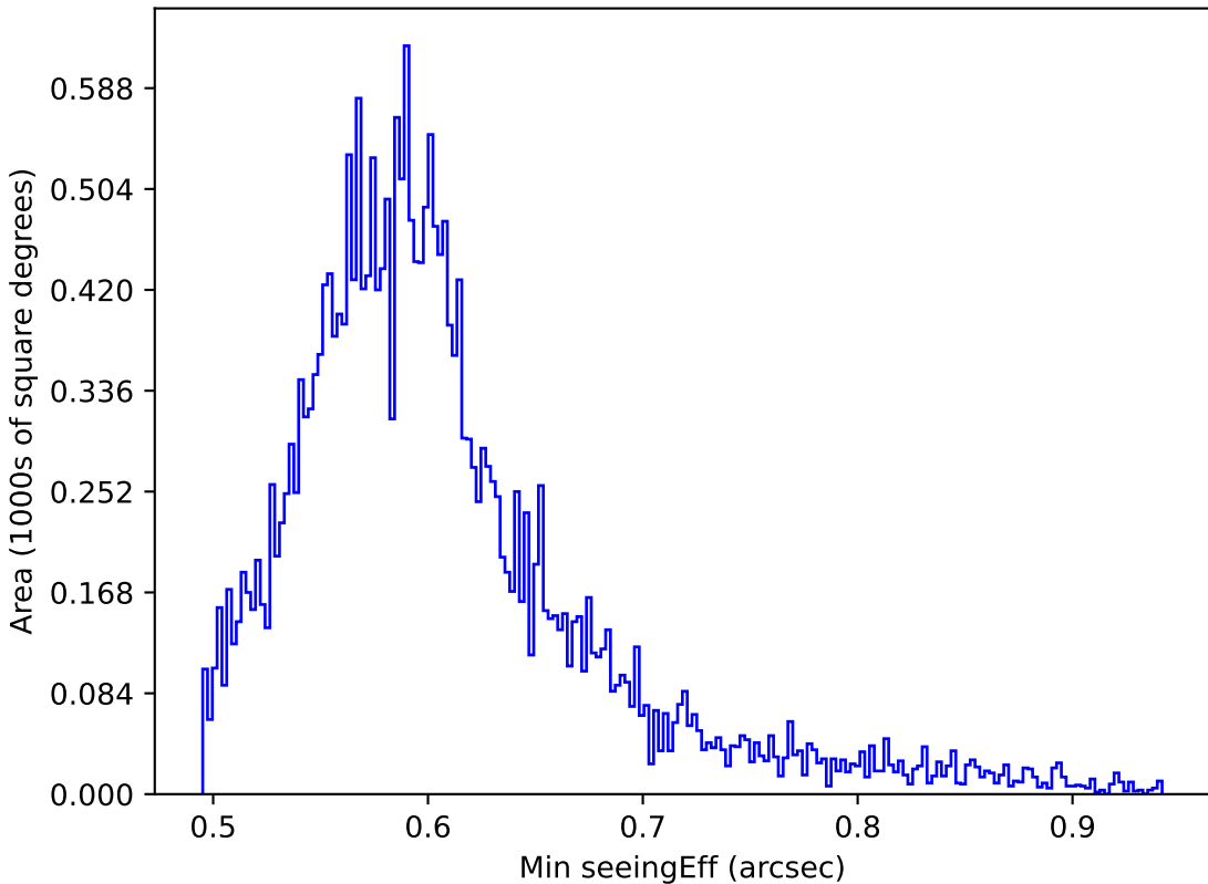
too_elab_r128_d2_gz_v3.4_10yrs All sky all bands: Min seeingEff
