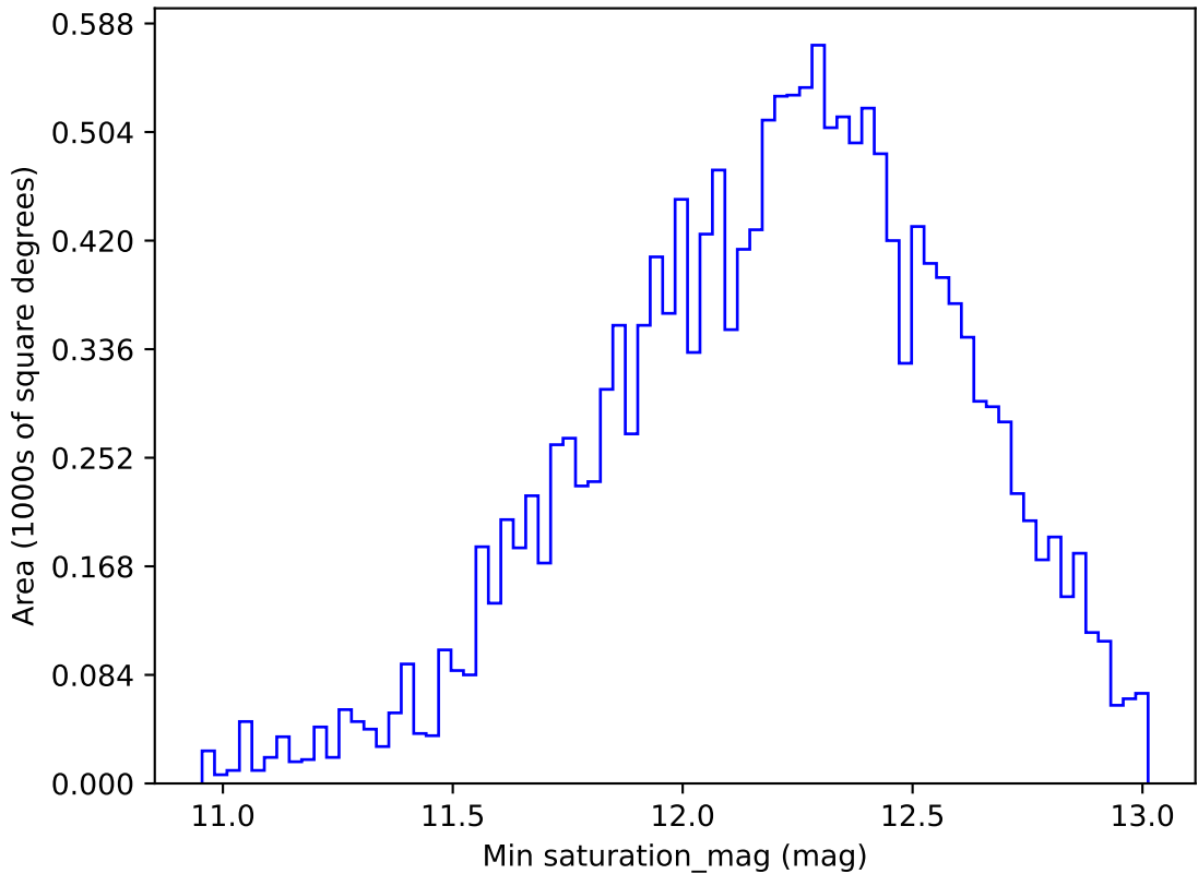
too_elab_r128_d2_gz_v3.4_10yrs WFD z band: Min saturation_mag
