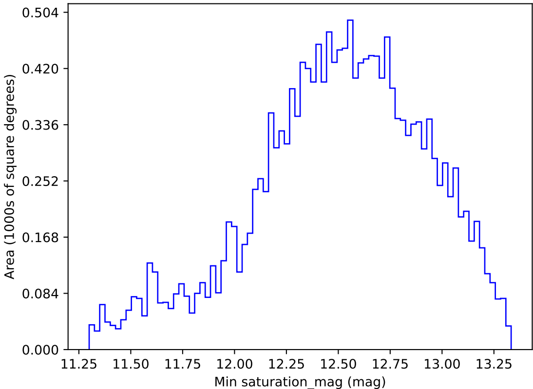
too_elab_r128_d2_gz_v3.4_10yrs WFD r band: Min saturation_mag
