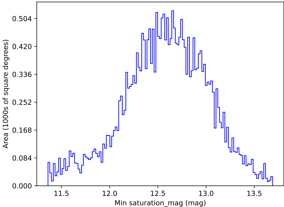
too_elab_r128_d2_gz_v3.4_10yrs All sky r band: Min saturation_mag
