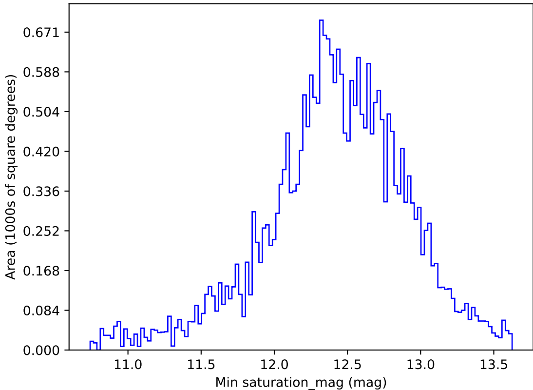
too_elab_r128_d2_gz_v3.4_10yrs All sky i band: Min saturation_mag
