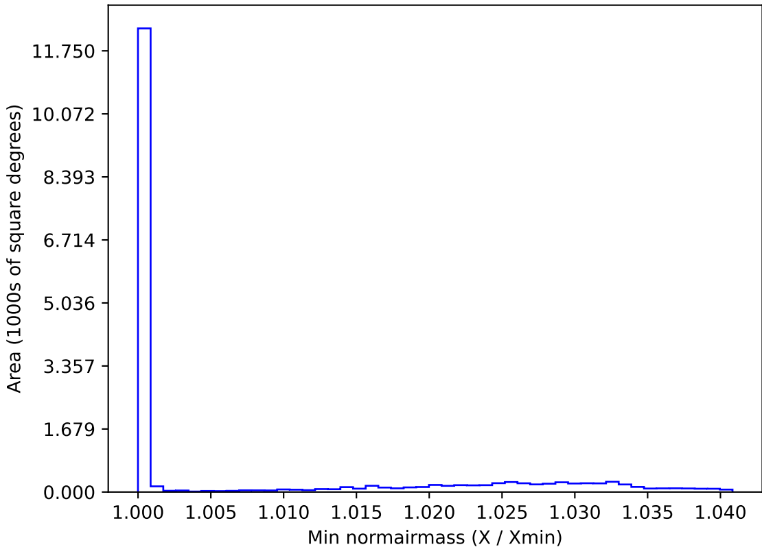
too_elab_r128_d2_gz_v3.4_10yrs WFD y band: Min normairmass
