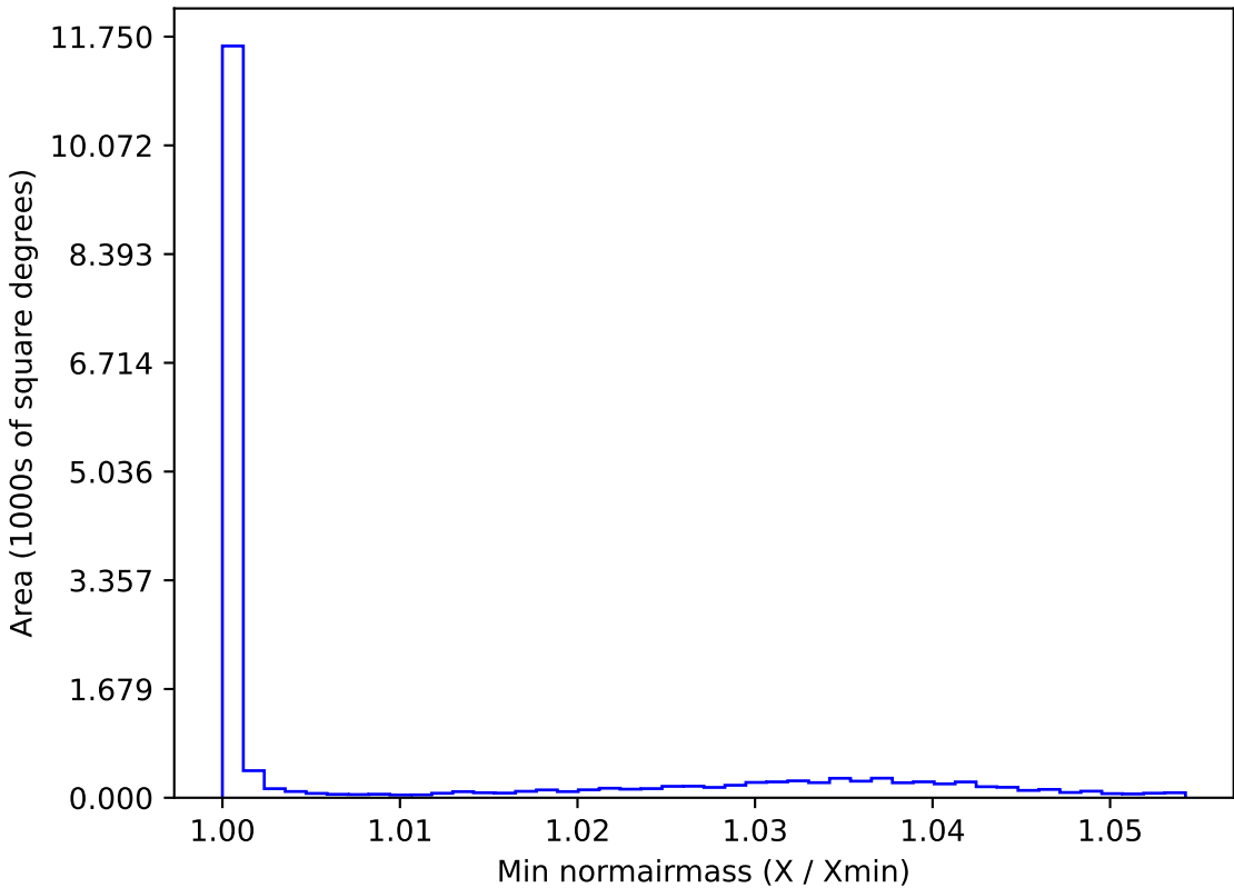
too_elab_r128_d2_gz_v3.4_10yrs WFD u band: Min normairmass
