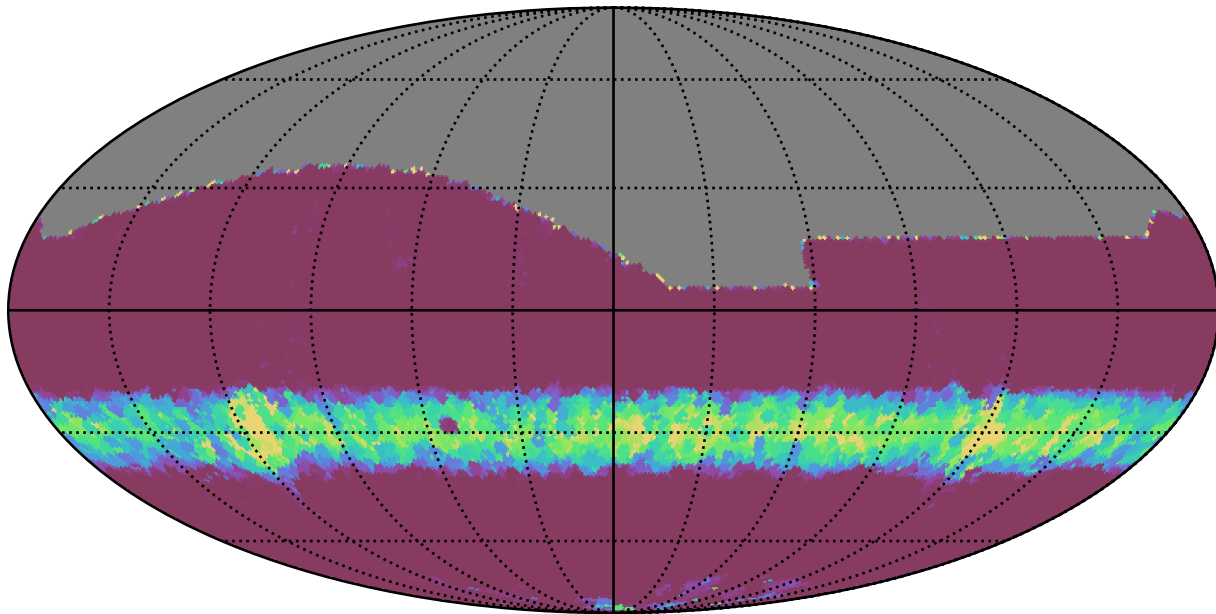
too_elab_r128_d2_gz_v3.4_10yrs All sky r band: Min normairmass
