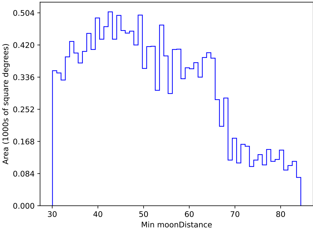
too_elab_r128_d2_gz_v3.4_10yrs WFD u band: Min moonDistance
