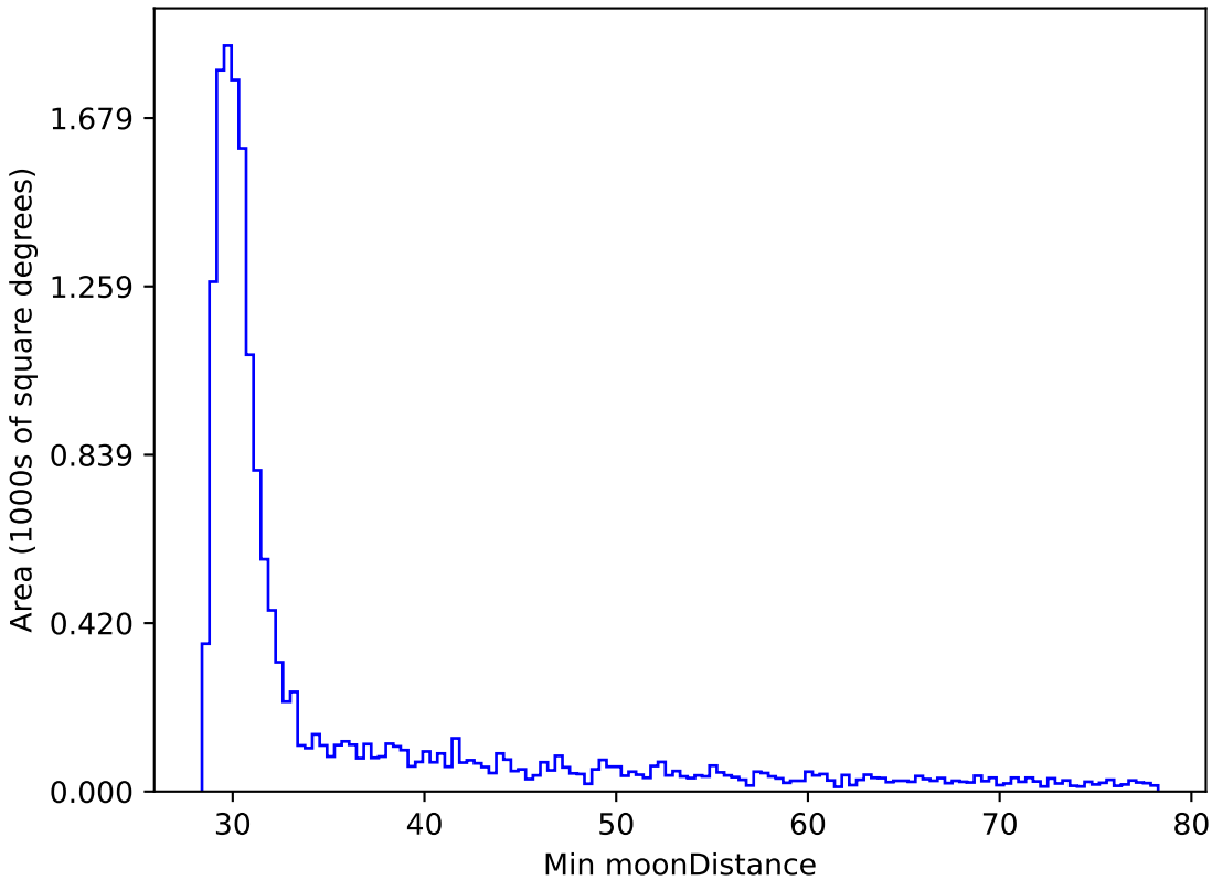
too_elab_r128_d2_gz_v3.4_10yrs WFD i band: Min moonDistance
