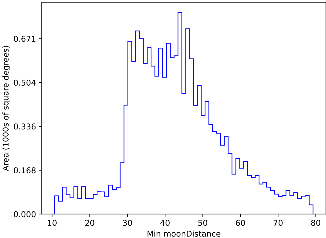
too_elab_r128_d2_gz_v3.4_10yrs WFD g band: Min moonDistance
